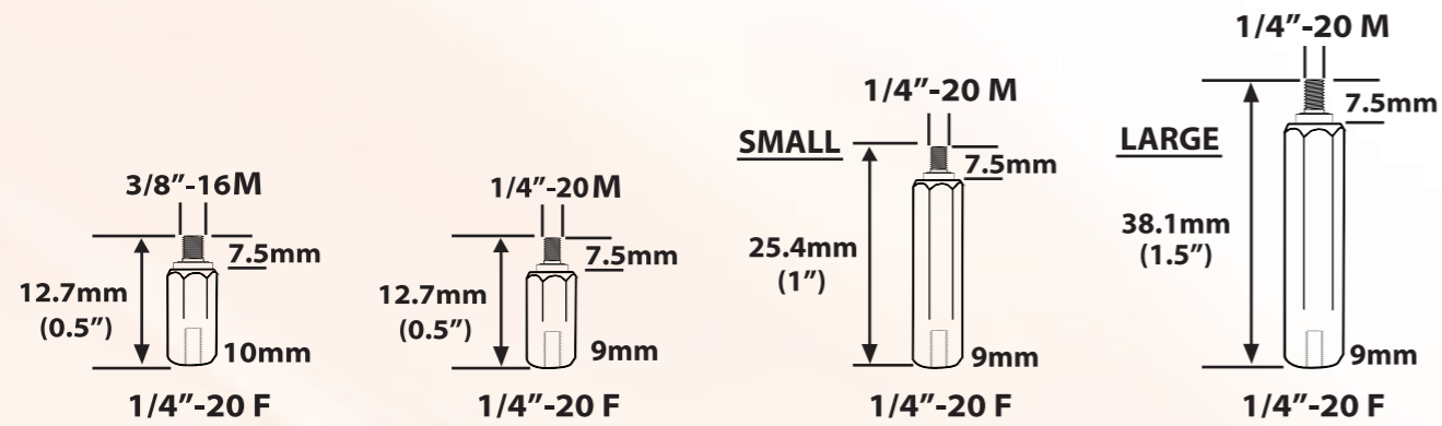
Screw Adapter
